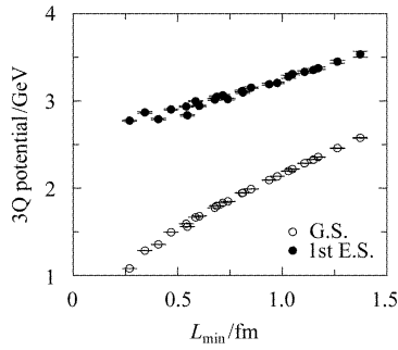
Fig.3. The lattice QCD results of the ground-state 3Q potential V_{3Q}^{g.s.} (open circles) and the 1st excited-state 3Q potential V_{3Q}^{e.s.} (filled circles) as the function of L_{min} .
