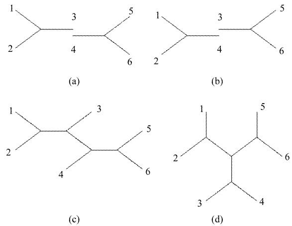
Fig.5. Color structures of six quark system.
