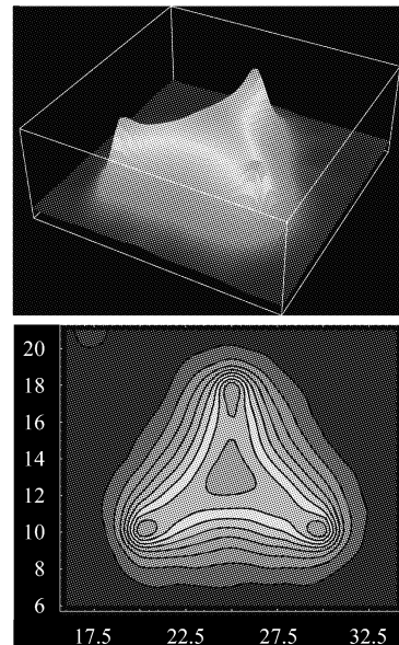
Fig.2. The lattice QCD result for the flux-tube profile in the spatially-fixed 3Q system.
