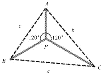
Fig.1. The flux-tube configuration of the 3Q system.
