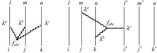
Fig.6. Three gluon exchange interactions.
