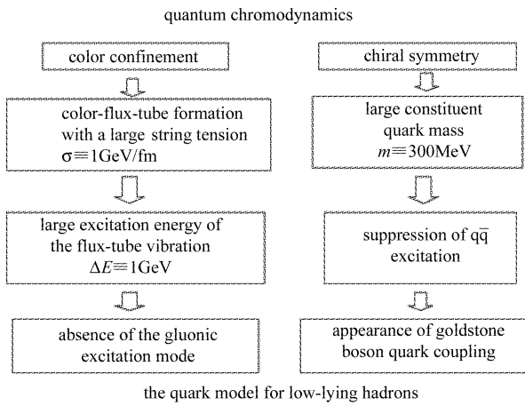
Fig.4. Connection from QCD to the quark model for low-lying hadrons.
