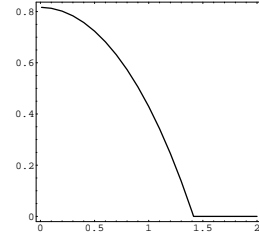
Fig. 2. v vs u according to Eq. (28).
