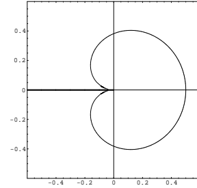
Fig. 1. Stability diagram for the galaxy distribution.
