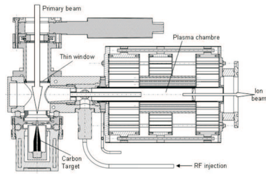
Fig. 1. Drawing of the TISS of SPIRAL I.
