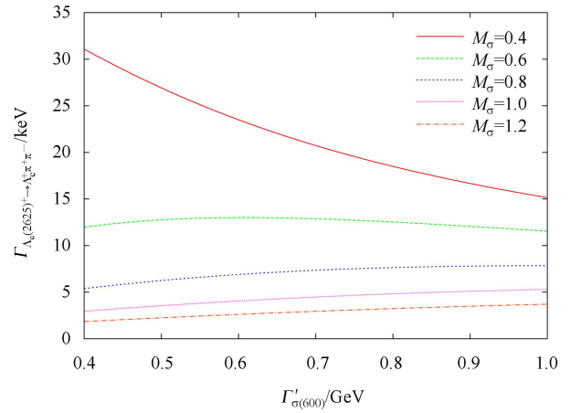
Fig. 1. The variation of the decay width of \Lambda_c(2625) \rightarrow \Lambda_c \pi^+ \pi^- with the resonance parameters of \sigma(600) .
