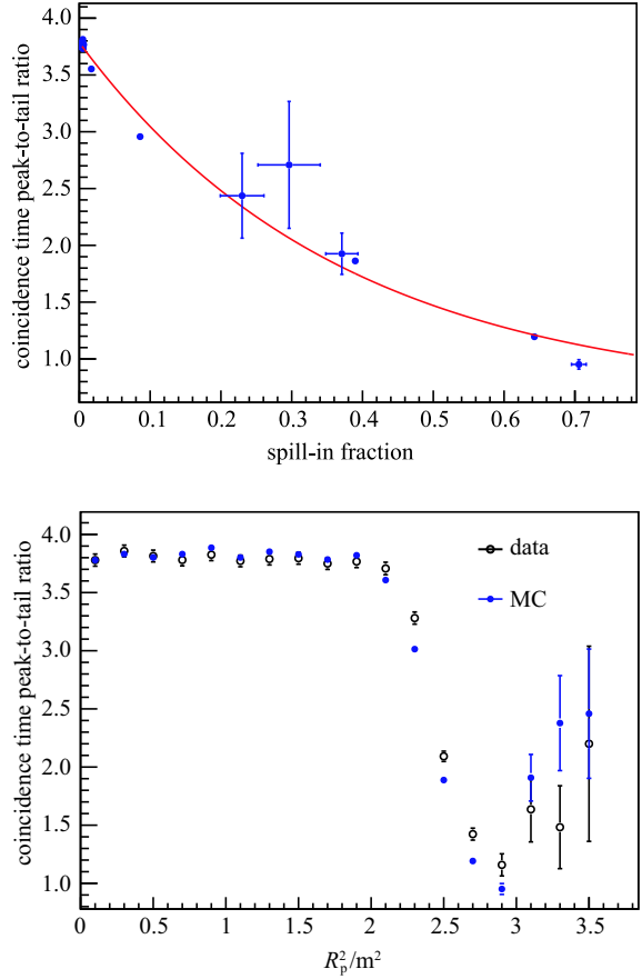
Fig. 13. (color online) Top: Points show the relation between true spill-in percentage and coincidence time peak-to-tail ratio in Monte Carlo simulation for event groupings at common R_{p,rec} . The peak-to-tail ratio compares IBD events in the (1,50) and (50,200) \mu\text{s} capture time regions. A curve is fitted to infer the spill-in fraction for the IBD candidate dataset. Bottom: The coincidence time peak-to-tail ratio in different bins along the radius. The spill-in percentage in each bin of data is predicted with the relation of spill-in and peak-to-tail ratio obtain from MC.
