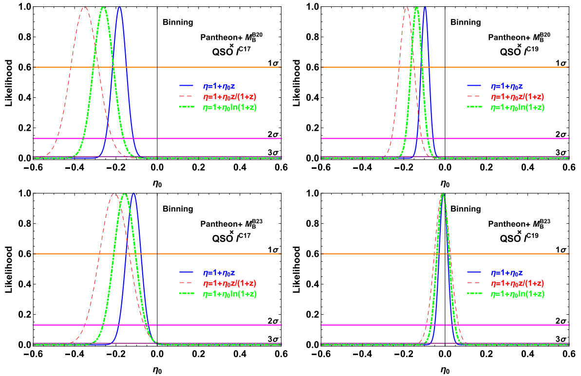
Fig. 4. (color online) Likelihood distribution functions obtained with the priors of M_B^{B20} (upper panel), M_B^{B23} (bottom panel), l^{C17} (left panel), and l^{C19} (right panel) in the binning method.
