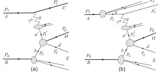
Fig. 3. (a): Coherent-resolved process in which the parton a' of a hadron-like photon emitted from nucleus A interacts with parton b of the target B via q-g Compton scattering, q-\bar{q} annihilation, and g-g fusion. (b): Incoherent-resolved process in which the parton a inside nucleus A emits a resolved virtual photon and parton a' of the resolved photon interacts with parton b inside target B in manner analogous to a hadron. After emitting the photon, nucleus A breaks up. In the process, photon emitter a represents a proton and quark for ordinary-incoherent photon emission (OIC) and ultra-incoherent photon emission (UIC), respectively.
