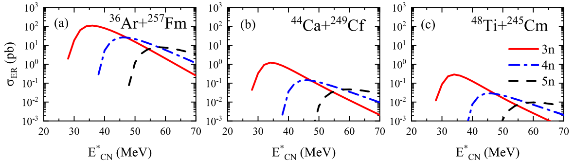
Fig. 2. (color online) Predicted ER cross sections for the reactions (a) ^{36}\text{Ar} + ^{257}\text{Fm} , (b) ^{44}\text{Ca} + ^{249}\text{Cf} , and (c) ^{48}\text{Ti} + ^{245}\text{Cm} . The calculated results for the 3n , 4n , and 5n channels are represented by solid, dash-dotted, and dashed lines, respectively.
