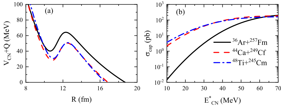
Fig. 3. (color online) (a) V_{CN} + Q values as a function of the distance between the centers of mass of the projectile and target nuclei for the reactions ^{36}\text{Ar} + ^{257}\text{Fm} , ^{44}\text{Ca} + ^{249}\text{Cf} , and ^{48}\text{Ti} + ^{245}\text{Cm} . (b) Capture cross sections for these reactions as a function of the excitation energy of the compound nucleus. The reactions ^{36}\text{Ar} + ^{257}\text{Fm} , ^{44}\text{Ca} + ^{249}\text{Cf} , and ^{48}\text{Ti} + ^{245}\text{Cm} are represented by solid, dashed and dash-dotted lines, respectively.
