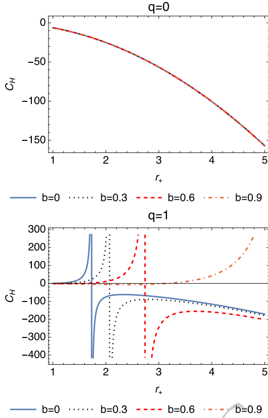
Fig. 3. (color online) The plots of C_H are governed by Eq. (27).
