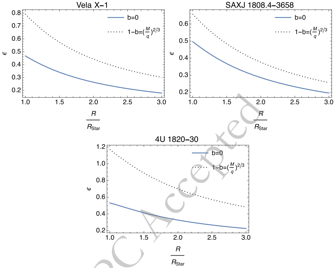
Fig. 13. (color online) These figures depict how the bending angle \epsilon changes with respect to R/R_{\text{star}} for the charged compact stars. Each graph compares the RN case ( b=0 ) with the Lorentz violation effect ( b \neq 0 ).
