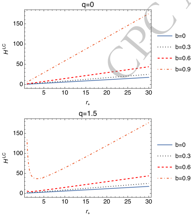
Fig. 8. (color online) The plots of H^{LC} are governed by Eq. (39).
