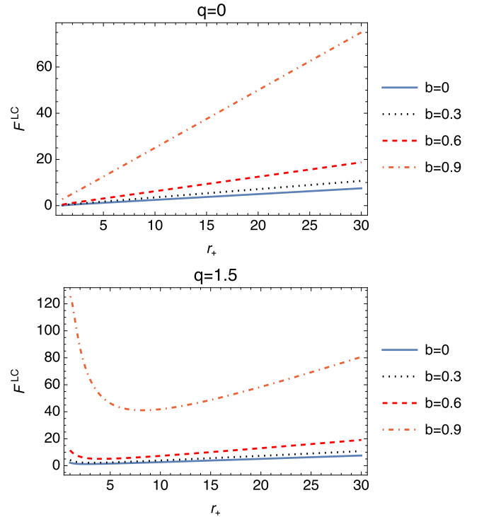
Fig. 6. (color online) The plots of F^{LC} are governed by Eq. (35).
