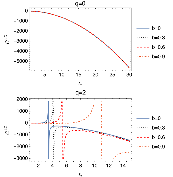
Fig. 10. (color online) The plots of C^{LC} are governed by Eq. (43).
