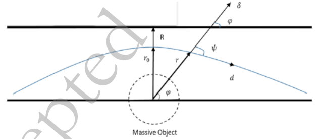
Fig. 12. (color online) The general bending of light geometry of the RI method
