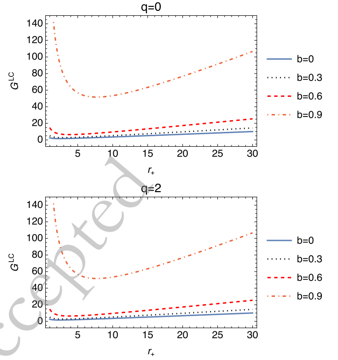
Fig. 9. (color online) The plots of G^{LC} are governed by Eq. (41).
