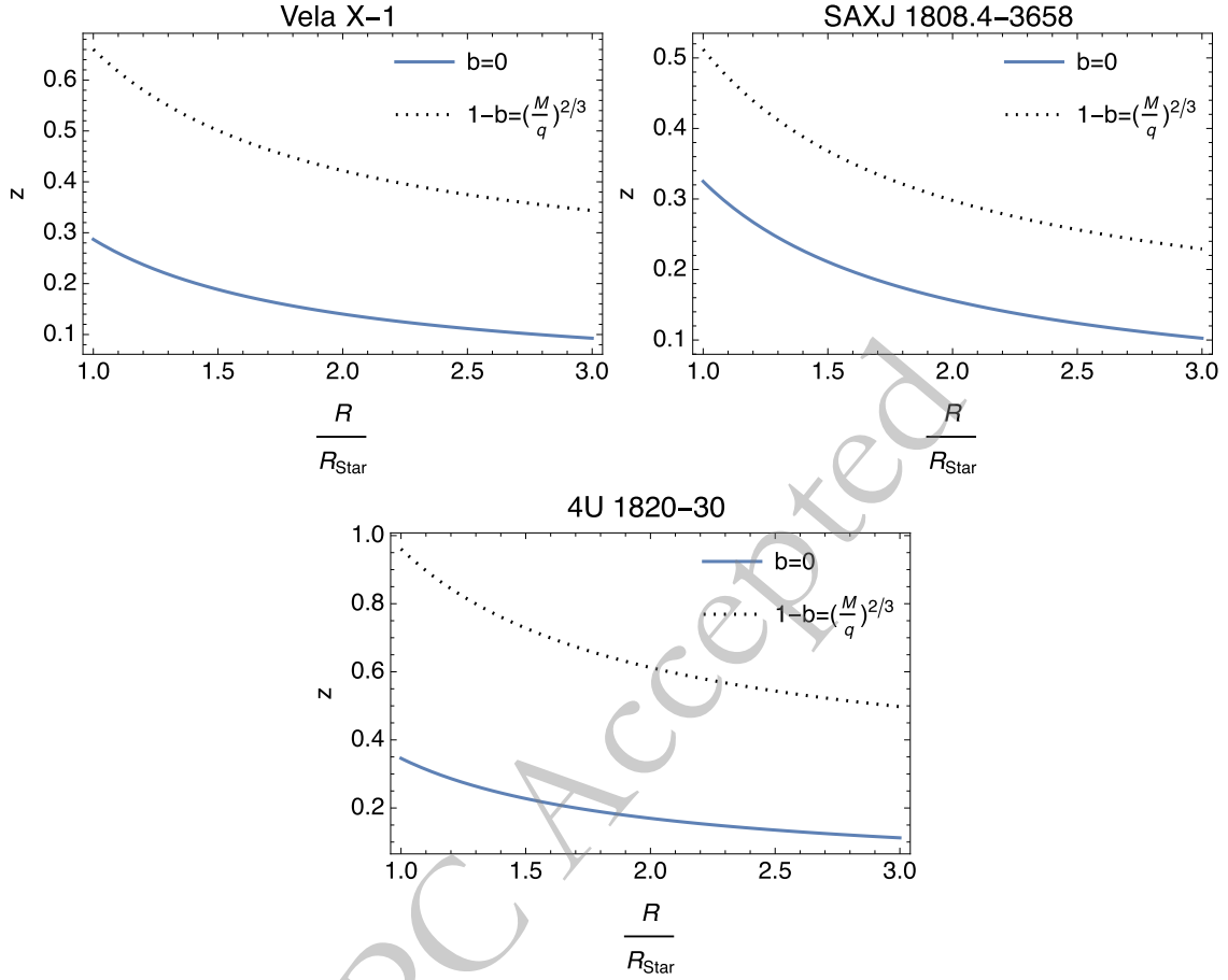
Fig. 14. (color online) The graphs show how the gravitational redshift parameter z evolves with respect to R/R_{\text{Star}} for the compact objects. Each graph includes trends for both the RN limit ( b = 0 ) and the Lorentz violation effect ( b \neq 0 ).
