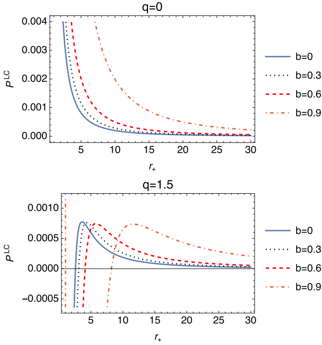
Fig. 7. (color online) The plots of p^{LC} are governed by Eq. (37).
