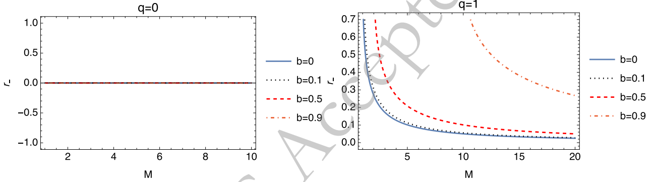
Fig. 2. (color online) Inner or Cauchy horizon ( r_- ) versus mass graph. The plots are governed by Eq. (5).
