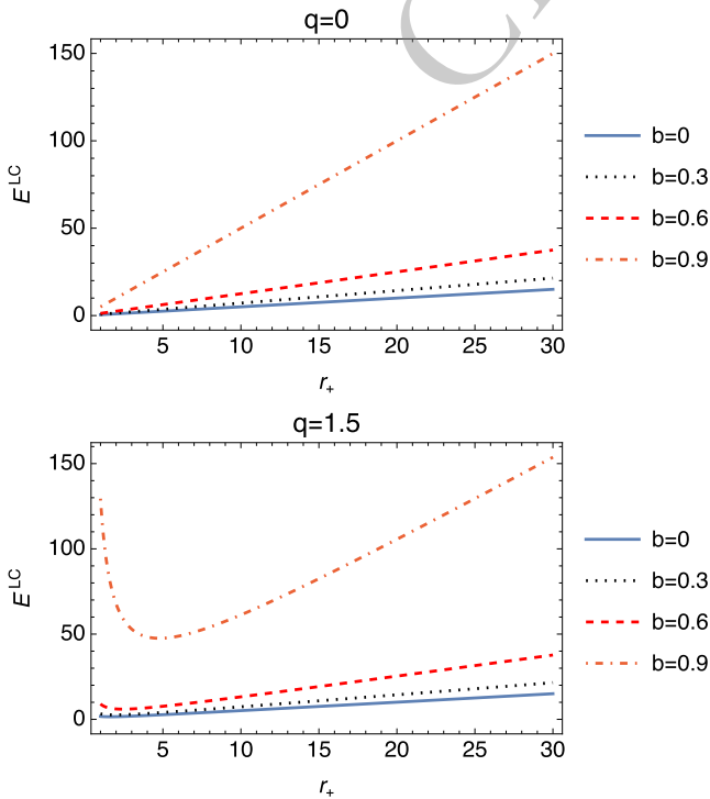
Fig. 5. (color online) The plots of E^{LC} are governed by Eq. (33).
