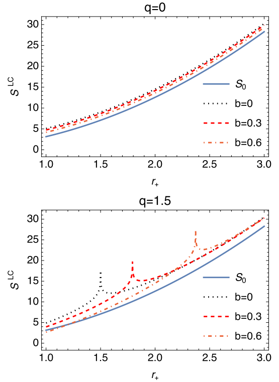
Fig. 4. (color online) The plots of S^{LC} are governed by Eq. (31) under the influence of maximum thermal fluctuations ( \alpha = 1 ).
