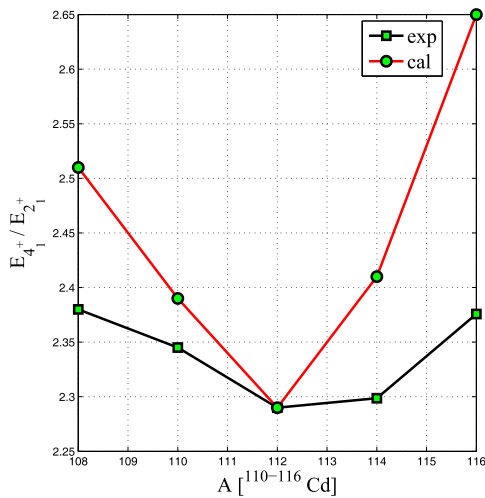
Fig. 2. (color online) Comparison of theoretical and experimental values of R_{4/2} = \frac{E(4_1^+)}{E(2_1^+)} and R_{0/2} = \frac{E(0_1^+)}{E(2_1^+)} for \text{Cd} isotopes.
