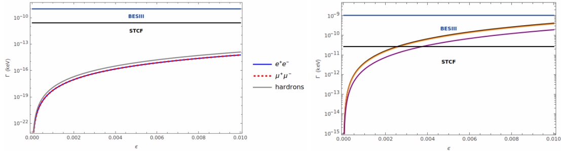
Fig. 6. (color online) Left: Decay width as a function of the kinetic mixing parameter \epsilon for the visible decays J/\psi \rightarrow U \rightarrow e^+e^- , J/\psi \rightarrow U \rightarrow \mu^+\mu^- , and J/\psi \rightarrow U \rightarrow \text{hadrons} . The dark blue and black horizontal lines represent the experimental limits from BESIII and STCF, respectively. Right: Decay width as a function of the kinetic mixing parameter \epsilon for the invisible decays J/\psi \rightarrow U \rightarrow \bar{\chi}_D\chi_D , J/\psi \rightarrow U \rightarrow \bar{\chi}_M\chi_M , and J/\psi \rightarrow U \rightarrow \varphi^\dagger\varphi , with \alpha_\chi = 0.05 and m_U/m_\chi = 3.0 . Both figures correspond to m_U = 1.0 \text{ GeV} .
