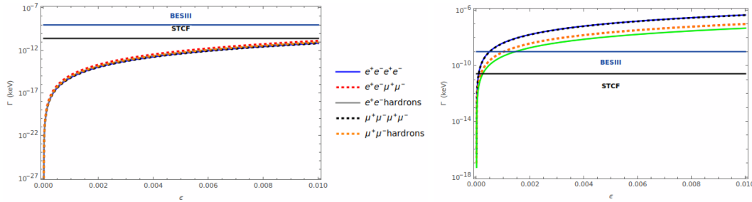
Fig. 9. (color online) Left panel: Decay width as a function of the kinetic mixing parameter \epsilon for the visible decay processes J/\psi \rightarrow l^+l^-U \rightarrow l^+l^-\mu^+\mu^- , J/\psi \rightarrow l^+l^-U \rightarrow l^+l^-e^+e^- , and J/\psi \rightarrow l^+l^-U \rightarrow l^+l^- hadrons. The dark blue and black horizontal lines represent the experimental limits from BESIII and STCF, respectively. Right panel: Decay width as a function of the kinetic mixing parameter \epsilon for the invisible decay processes J/\psi \rightarrow l^+l^-U \rightarrow l^+l^-\bar{\chi}_D\chi_D , J/\psi \rightarrow l^+l^-U \rightarrow l^+l^-\bar{\chi}_M\chi_M , and J/\psi \rightarrow l^+l^-U \rightarrow l^+l^-\varphi^\dagger\varphi , with \alpha_\chi = 0.05 and m_U/m_\chi = 3.0 . Both panels correspond to m_U = 1.0 GeV.
