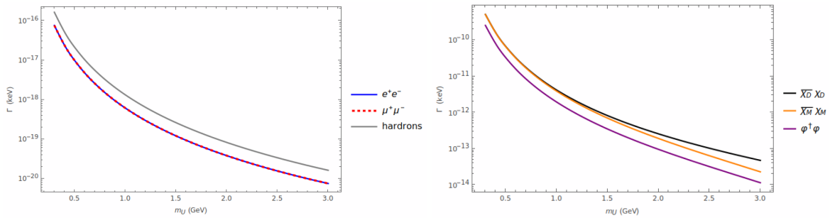
Fig. 7. (color online) Left: Decay width as a function of the dark photon mass m_U for the visible decay processes J/\psi \rightarrow U \rightarrow e^+e^- , \mu^+\mu^- , and hadrons. Right: Decay width as a function of the dark photon mass m_U for the invisible decay processes J/\psi \rightarrow U \rightarrow \bar{\chi}_D\chi_D , \bar{\chi}_M\chi_M , and \varphi^\dagger\varphi , with \alpha_\chi = 0.05 and m_U/m_\chi = 3.0 . In both figures, \epsilon = 10^{-3} .
