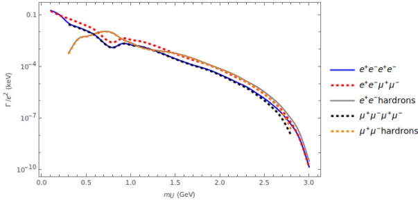
Fig. 8. (color online) Decay width \Gamma(J/\psi \rightarrow l^+l^-U \rightarrow l^+l^-X) divided by \epsilon^2 as a function of the dark photon mass m_U , for the four-body final-state decay processes: J/\psi \rightarrow l^+l^-U \rightarrow l^+l^-\mu^+\mu^- , J/\psi \rightarrow l^+l^-U \rightarrow l^+l^-e^+e^- , and J/\psi \rightarrow l^+l^-U \rightarrow l^+l^- hadrons.
