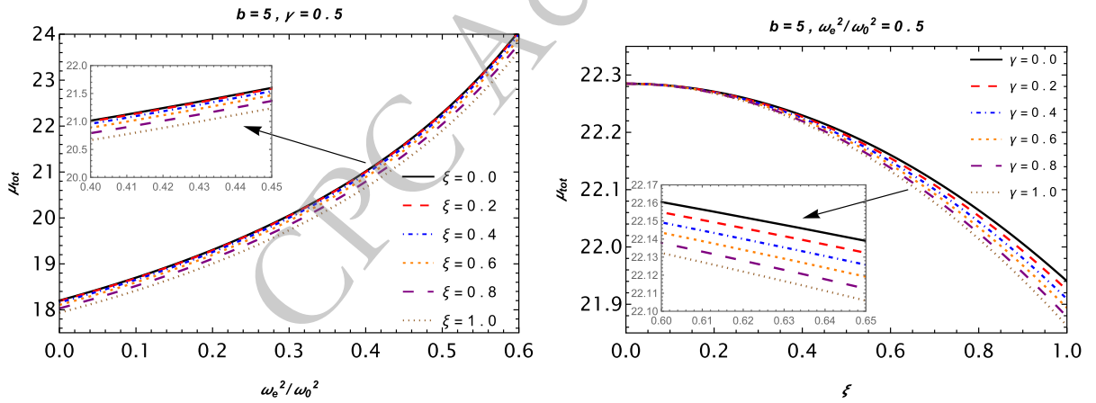
Fig. 13. (color online) Left panel: The total magnification as a function of the uniform plasma frequency for different values of the \xi parameter, with other parameters fixed at b = 5 and \gamma = 0.5 . The right panel shows the dependence of the total magnification on the \xi parameter for different values of the \gamma parameter. Here, we set b = 5 and \omega_c^2/\omega_0^2 = 0.5 .
