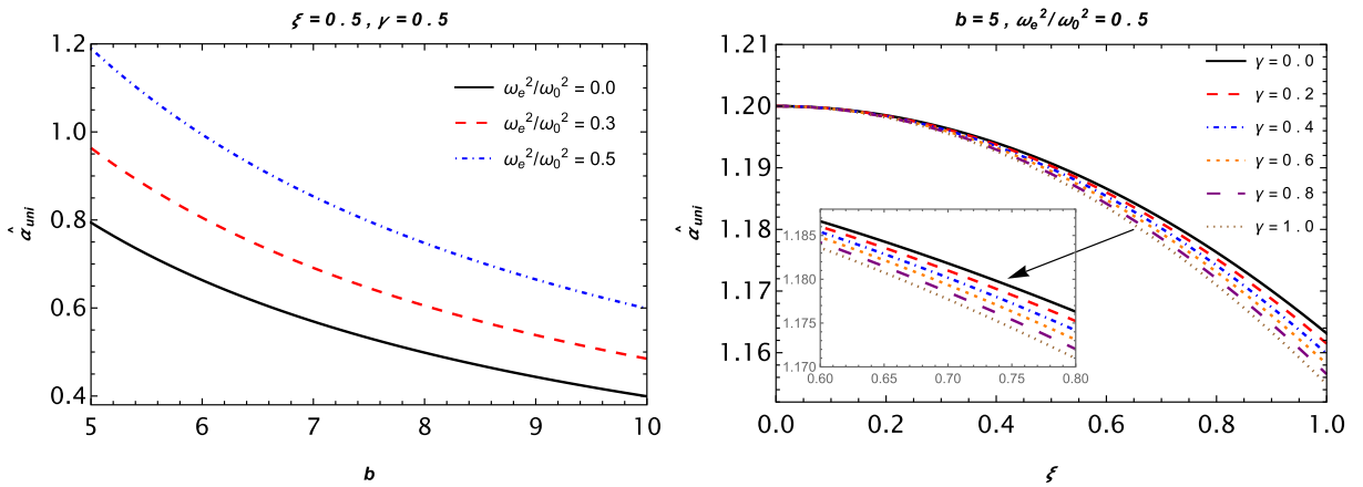
Fig. 10. (color online) The left panel shows the deflection angle as a function of the impact parameter for different values of the uniform plasma frequency. Here, we set the spacetime parameters as \xi = 0.5 and \gamma = 0.5 . The right panel illustrates the dependence of the deflection angle on the \zeta parameter for different values of the \gamma parameter. The impact parameter and the plasma frequency were fixed for this panel, i.e., b = 5 and \omega_e^2/\omega_0^2 = 0.5 .
